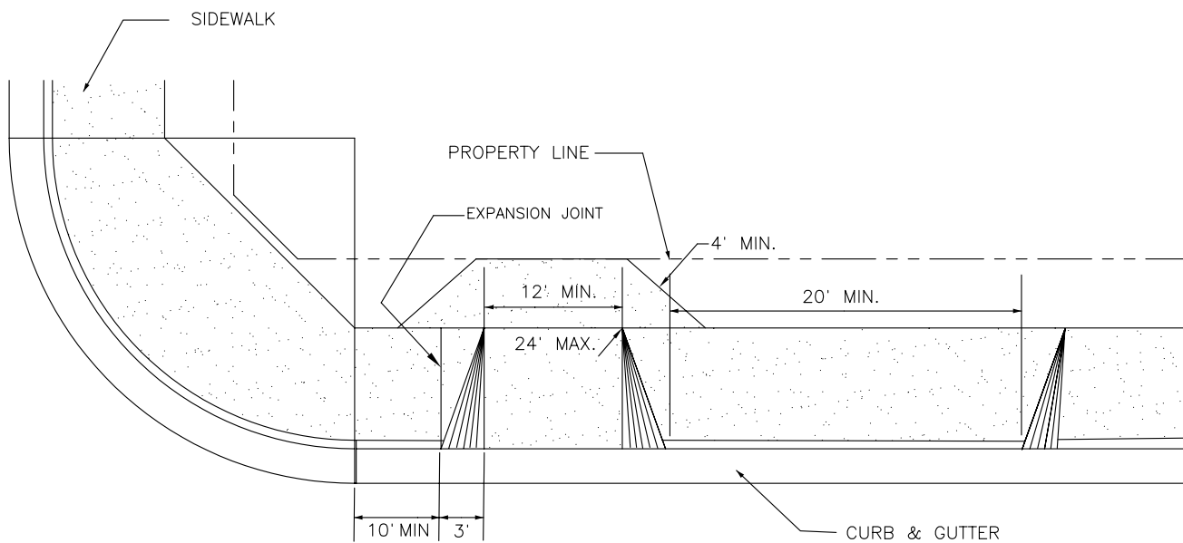
STANDARD CURB, GUTTER & NON-ADJACENT SIDEWALK
