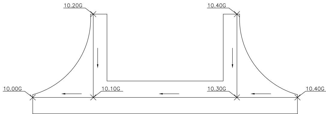
TYPICAL DRAINAGE FOR LOCAL STREET (GUTTER GRADES)
