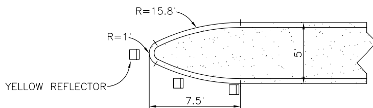
ISLAND NOSE DETAIL
