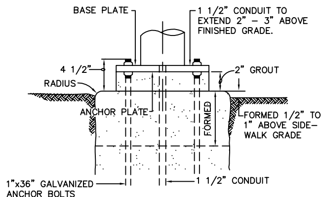
BASE DETAIL
