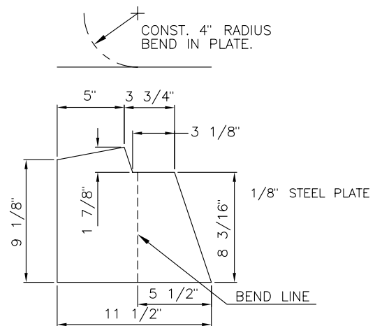
THROAT SIDEPLATE
